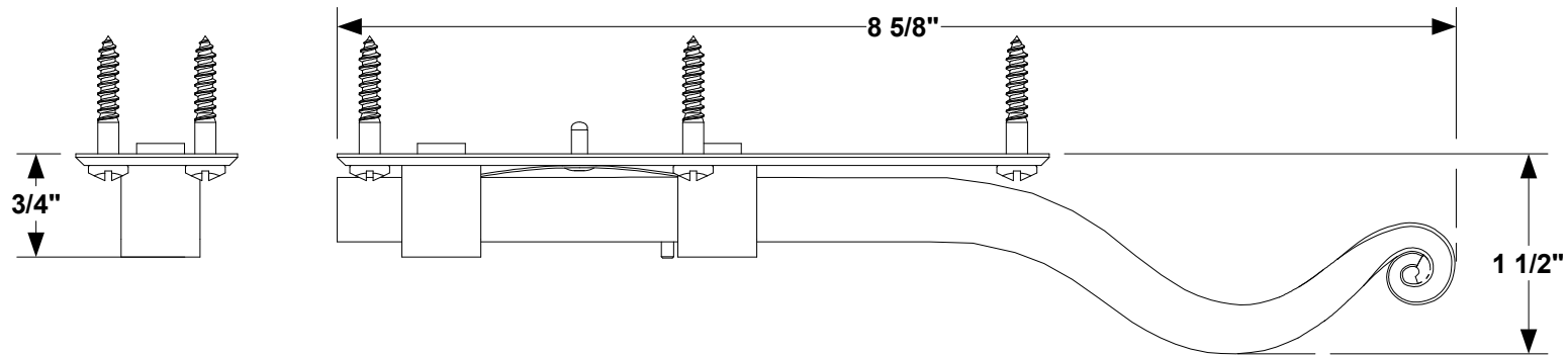
1 TOP VIEW
