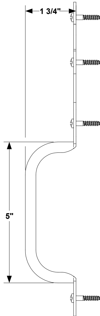
2 SIDE VIEW
