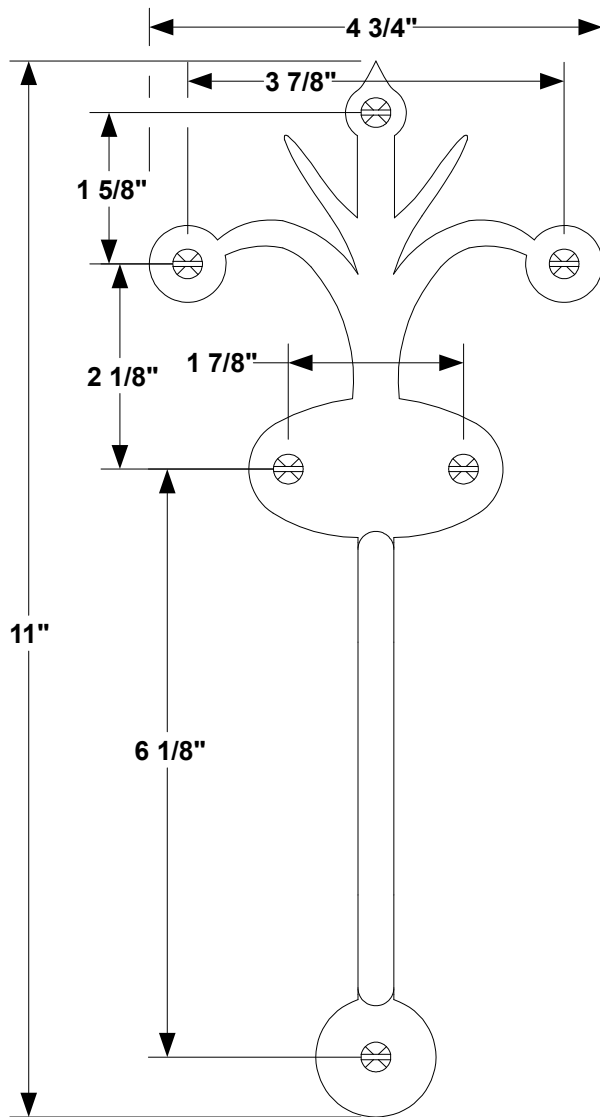
1 FRONT VIEW
