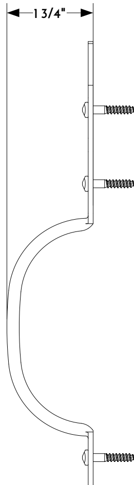
2 SIDE VIEW
