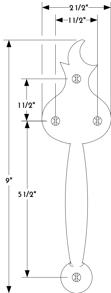
1 FRONT VIEW
