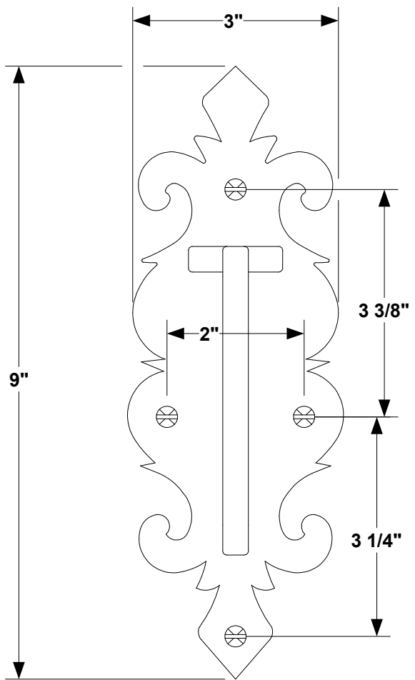
1 FRONT VIEW
