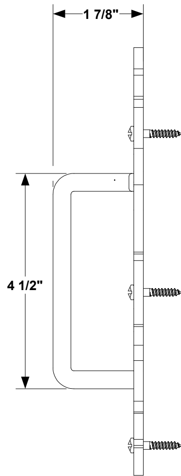
2 SIDE VIEW
