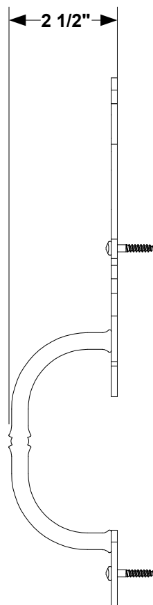
2 SIDE VIEW
