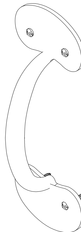
3 ISOMETRIC VIEW
