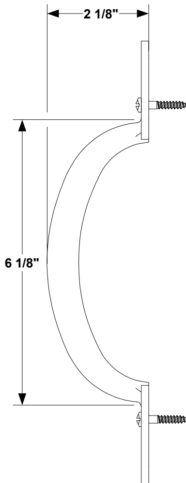
2 SIDE VIEW
