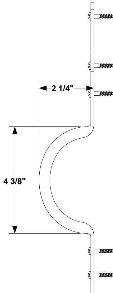
2 SIDE VIEW
