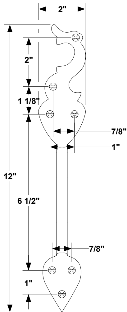
1 FRONT VIEW
