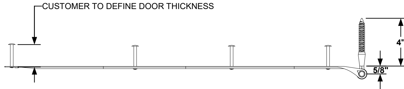
2 TOP VIEW
