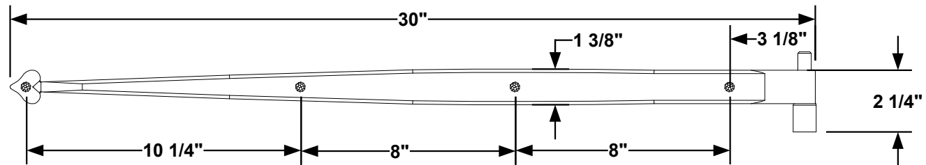
1 FRONT VIEW
