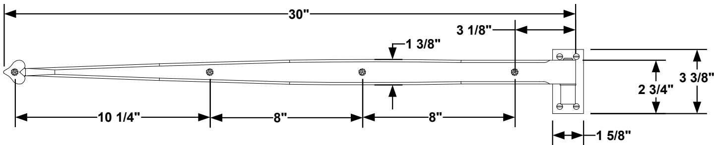
1 FRONT VIEW
