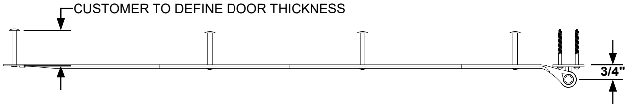
2 TOP VIEW
