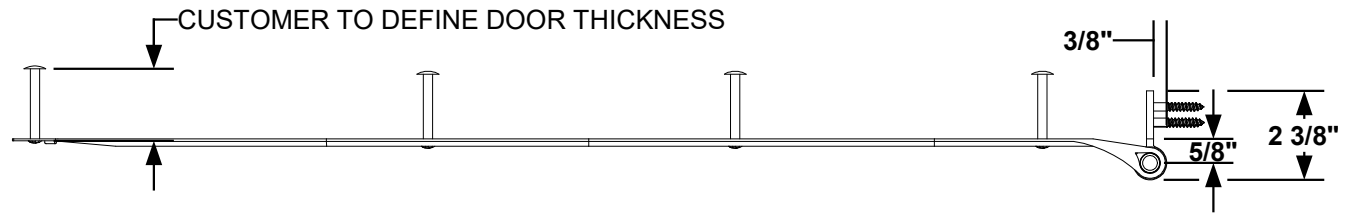
2 TOP VIEW
