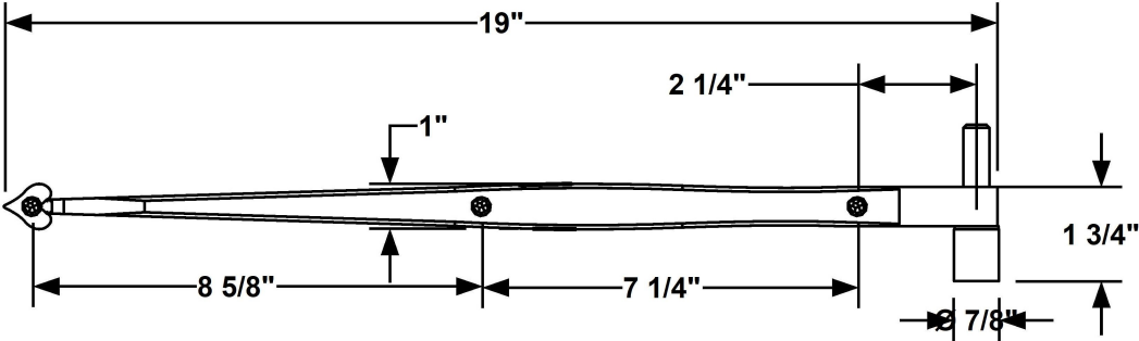
2 TOP VIEW
