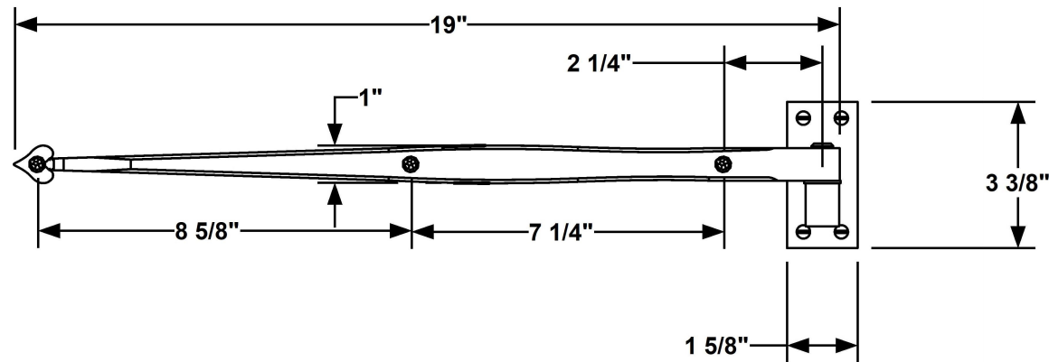
1 FRONT VIEW
