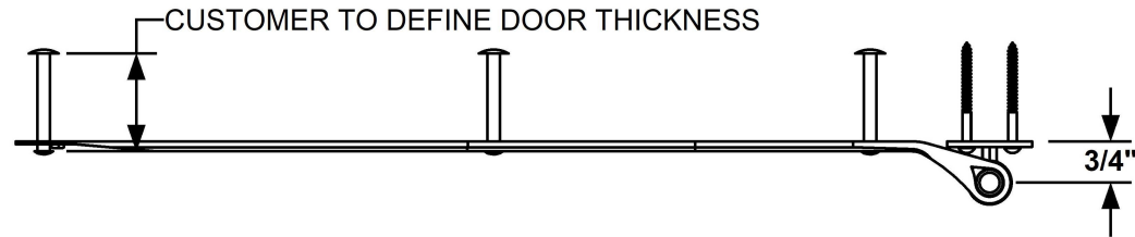
2 TOP VIEW
