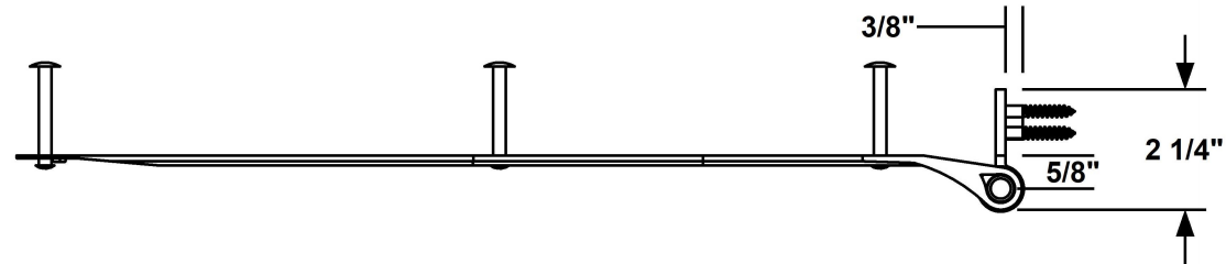
2 TOP VIEW
