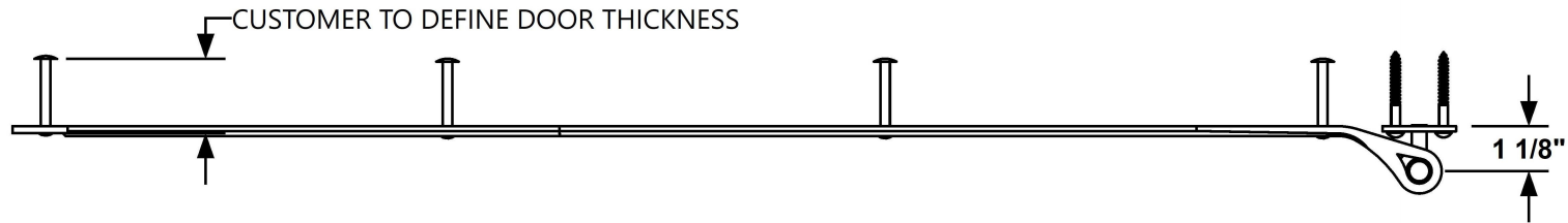
2 TOP VIEW
