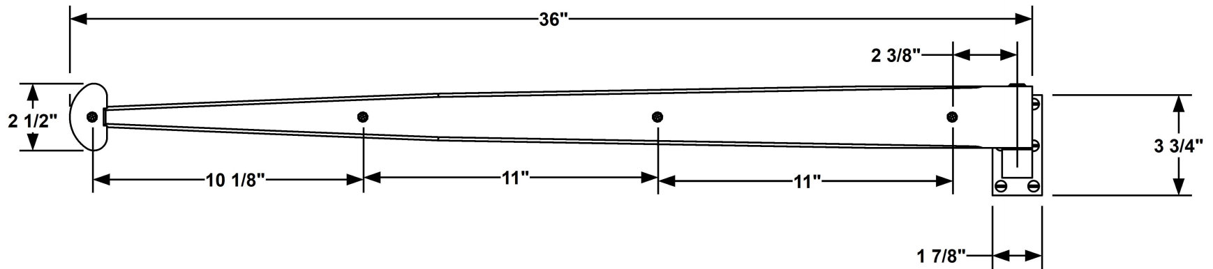
1 FRONT VIEW
