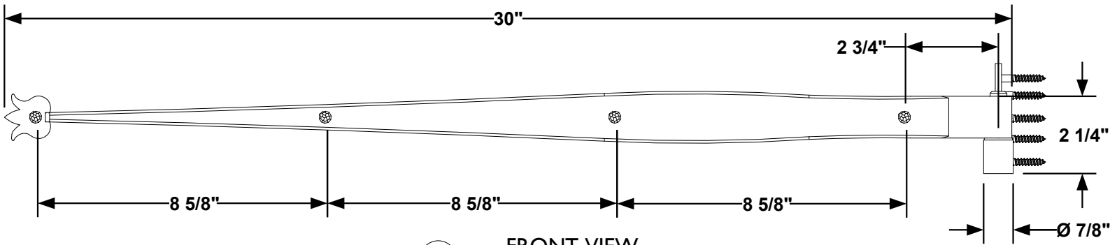
1 FRONT VIEW
