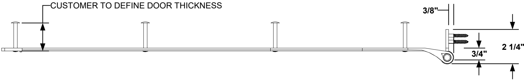
2 TOP VIEW
