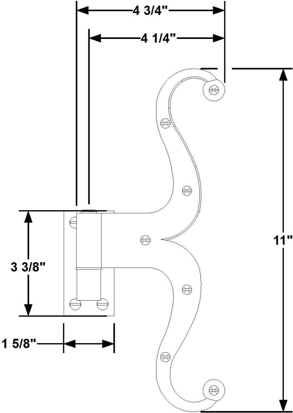
1 FRONT VIEW
