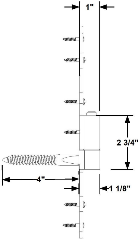
2 TOP VIEW
