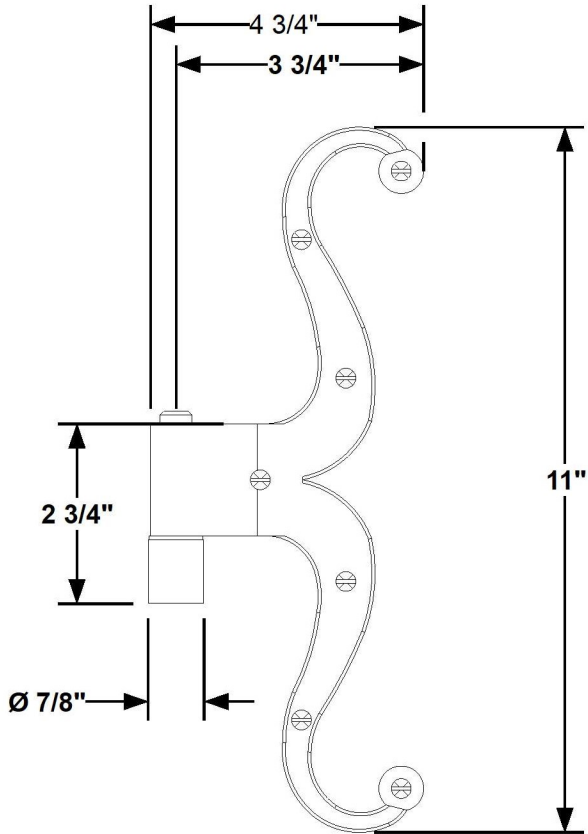
1 FRONT VIEW
