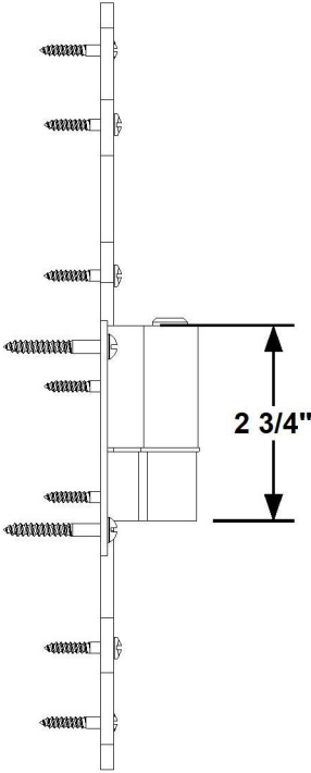
2 TOP VIEW
