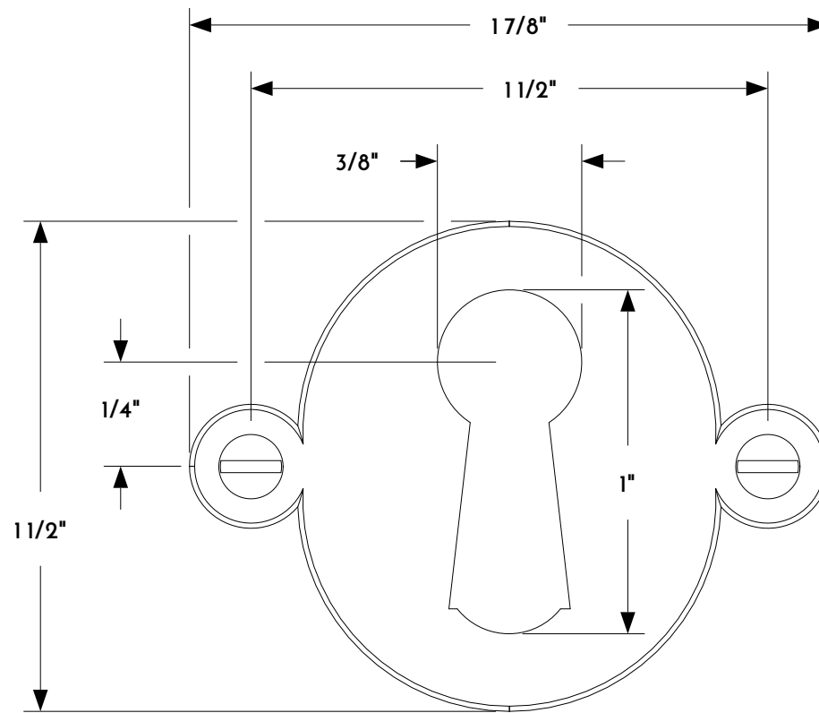
1 FRONT VIEW
