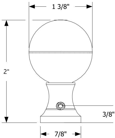
1 FRONT VIEW
