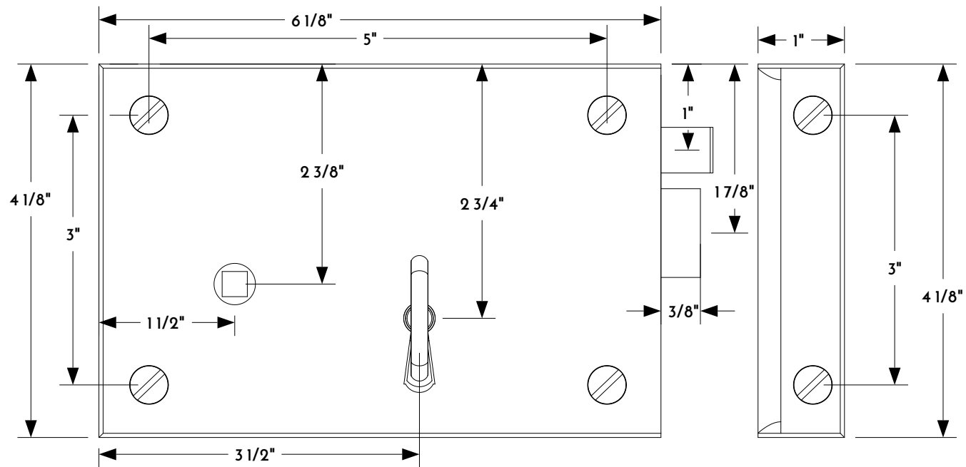
2 FRONT VIEW
