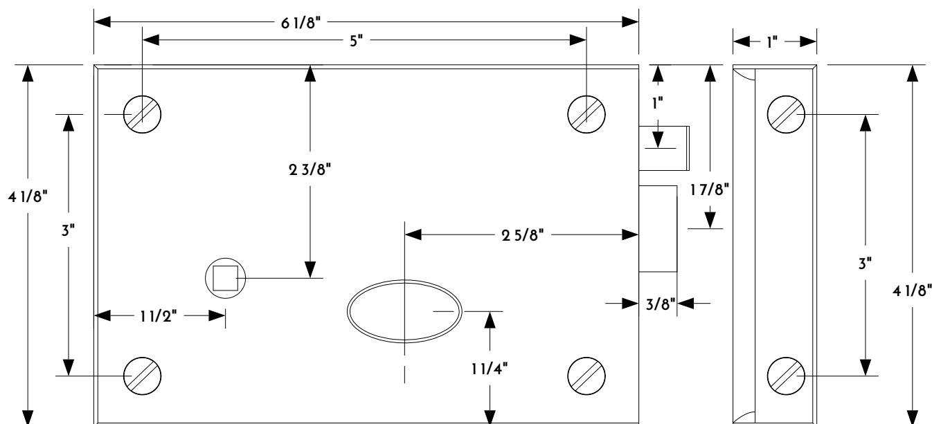
2 FRONT VIEW
