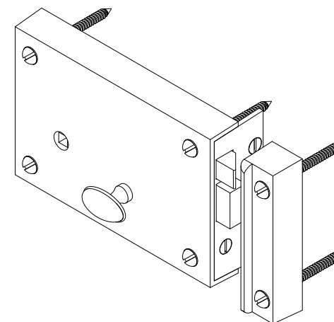
3 ISOMETRIC VIEW
