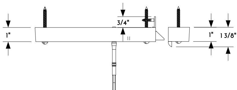
1 TOP VIEW
