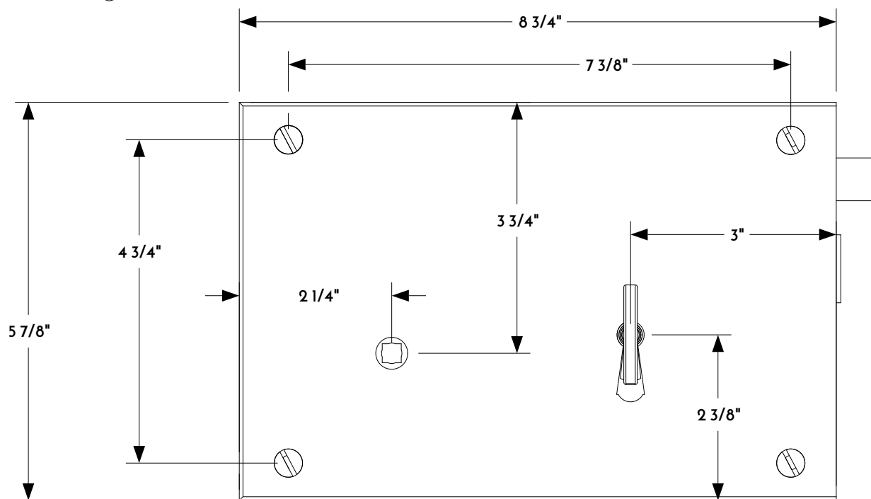
2 FRONT VIEW
