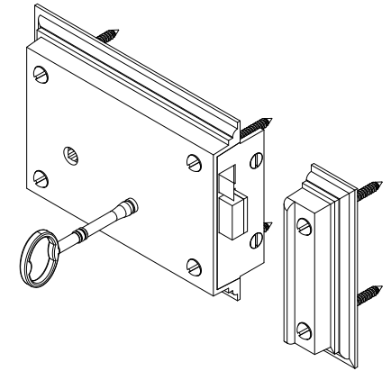
3 ISOMETRIC VIEW
