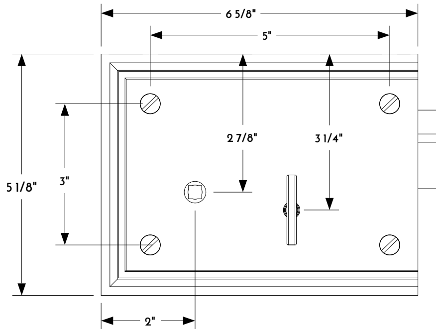
2 FRONT VIEW
