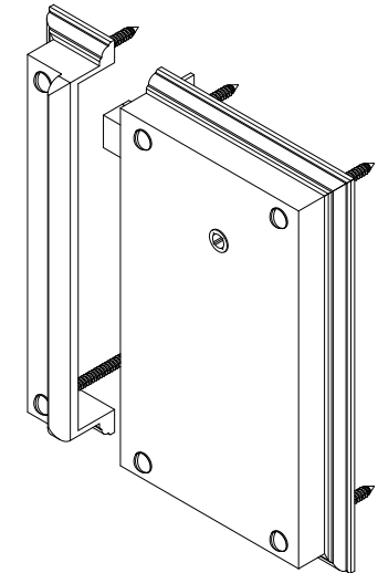
3 ISOMETRIC VIEW
