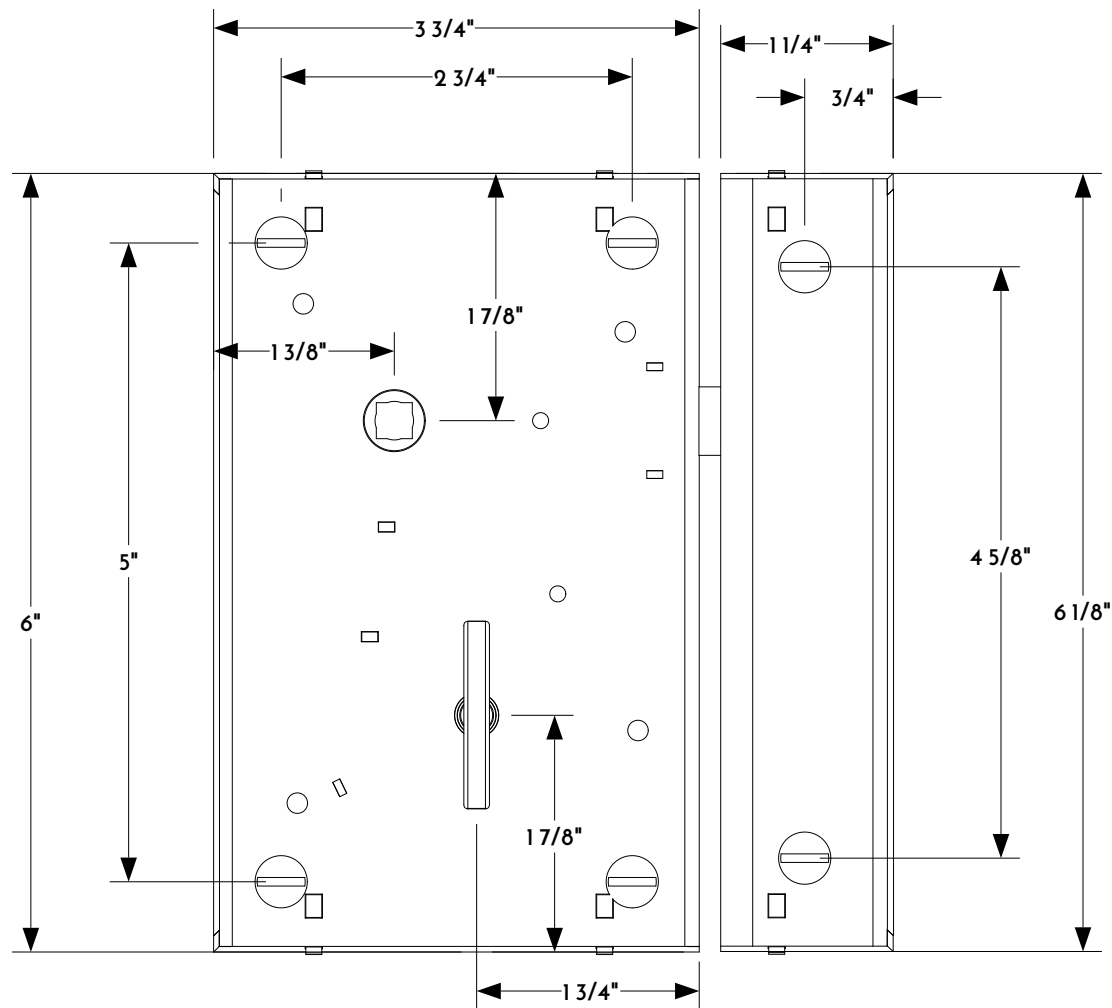
2 FRONT VIEW
