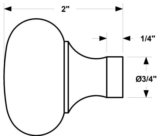
2 SIDE VIEW
