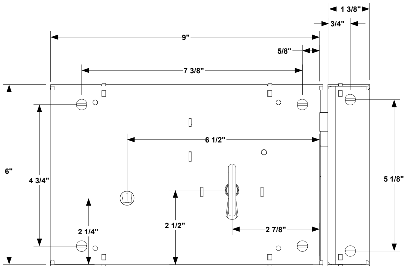
2 FRONT VIEW
