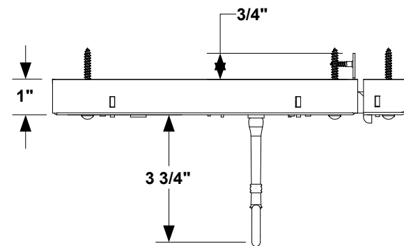
1 TOP VIEW
