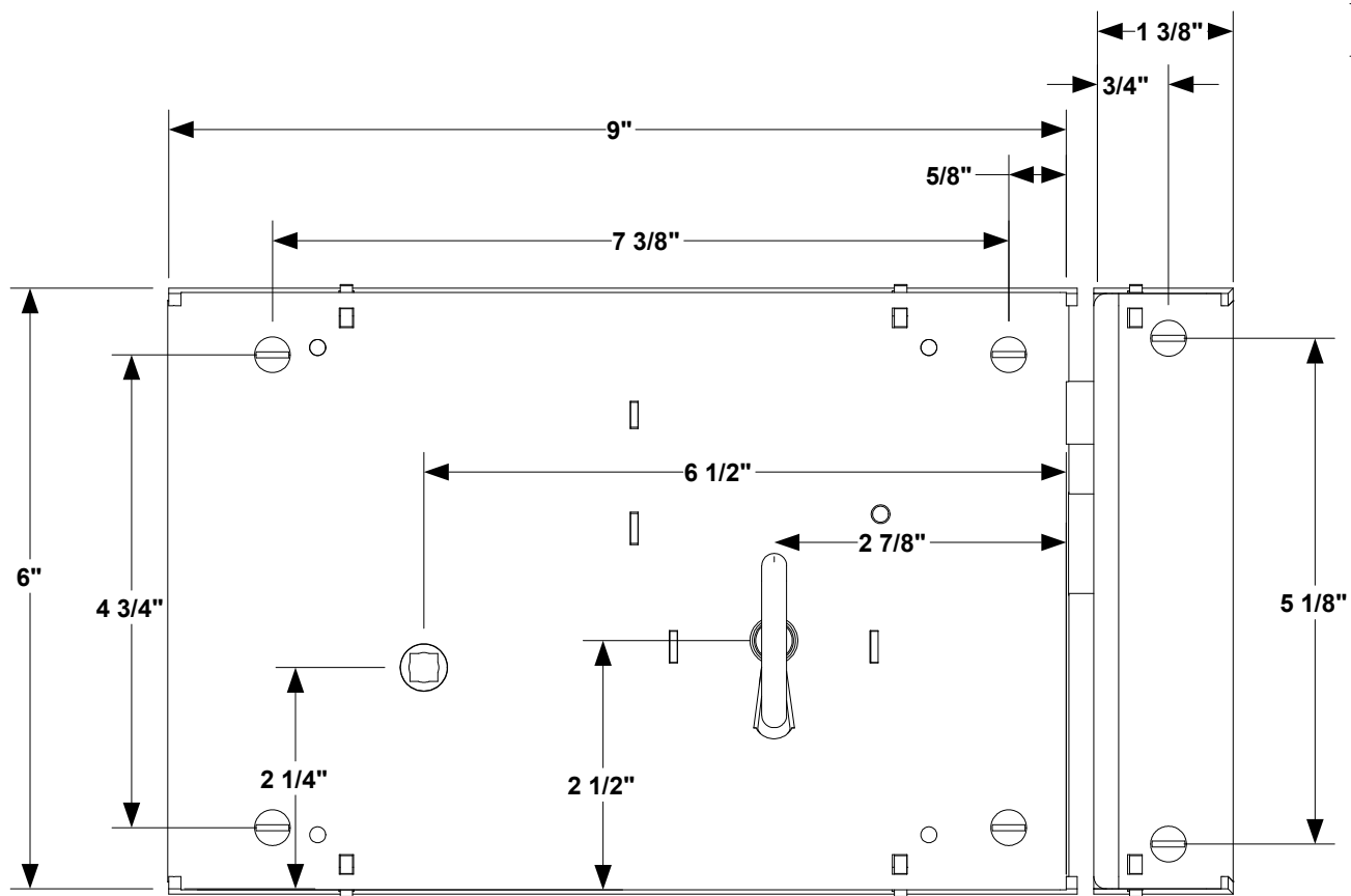
2 FRONT VIEW
