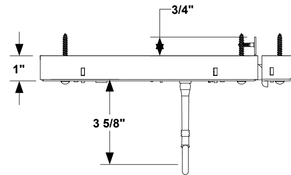
1 TOP VIEW
