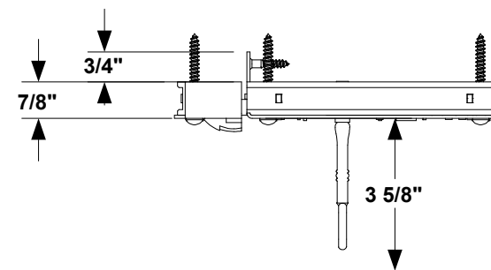
1 TOP VIEW
