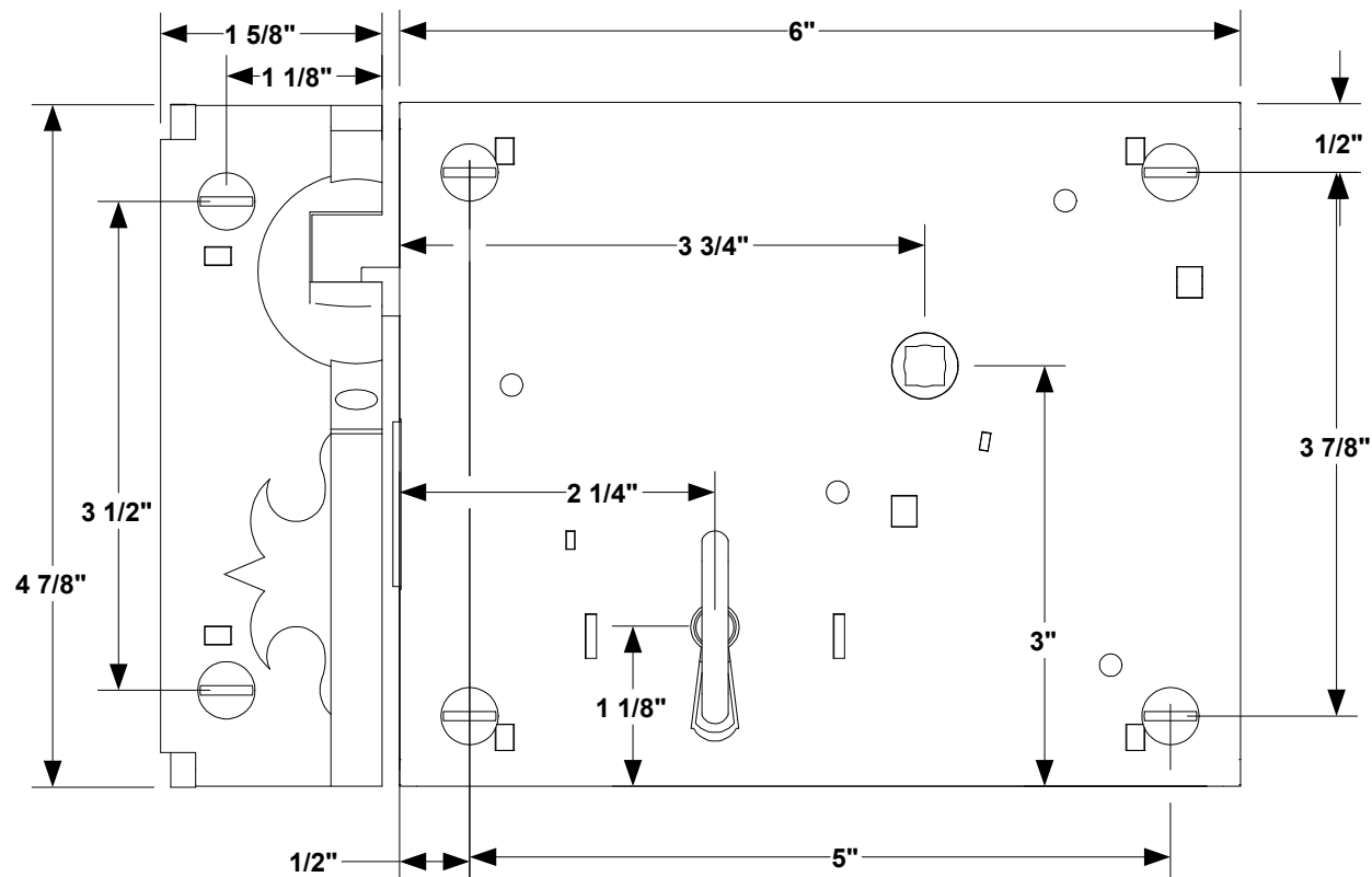
2 FRONT VIEW
