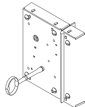
3 ISOMETRIC VIEW
